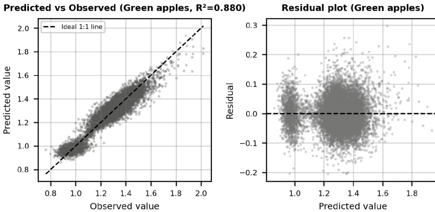
Figure 4. Predicted versus observed values (left) and residual plot (right) for the green apple cultivar model ( R^2=0.880 )
